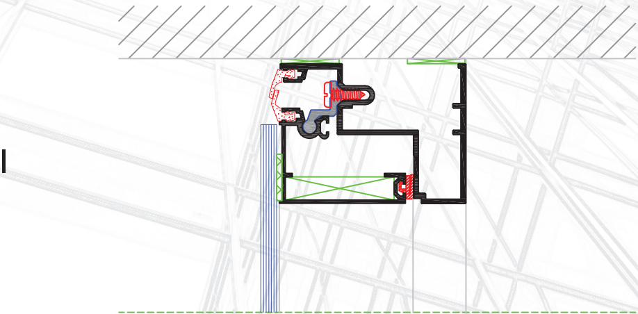
CORTE VERTICAL
