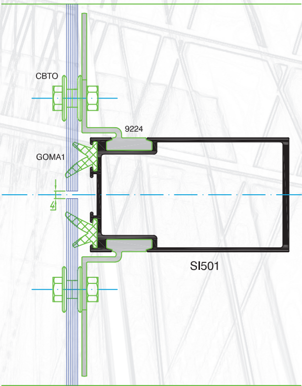
CORTE VERTICAL
