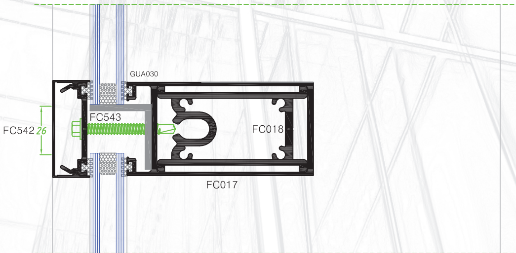
CORTE VERTICAL
