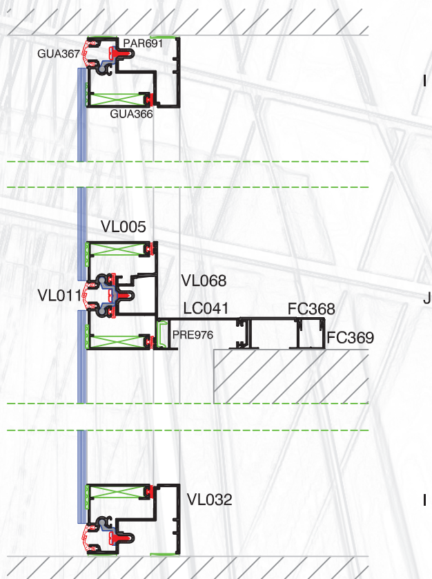
CORTE VERTICAL
