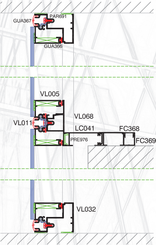
CORTE VERTICAL
