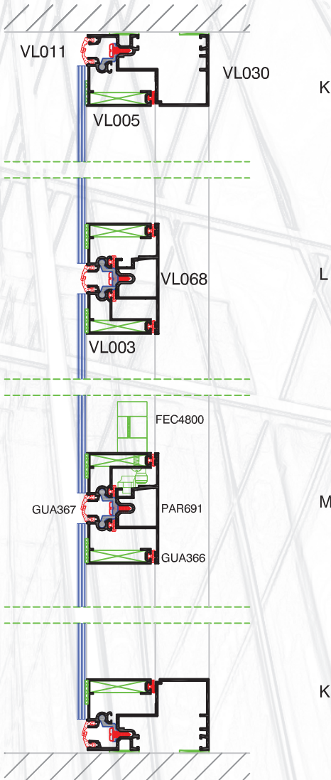
CORTE VERTICAL
