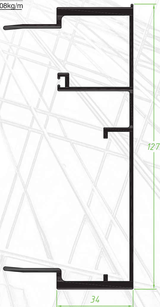
Tapa travesa central modular
