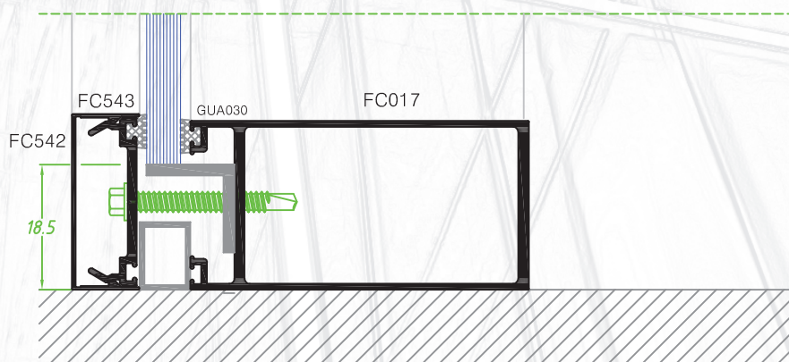
CORTE VERTICAL
