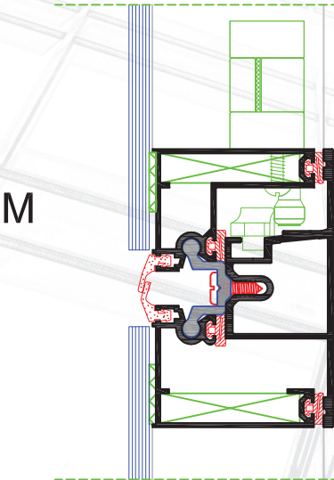
CORTE VERTICAL
