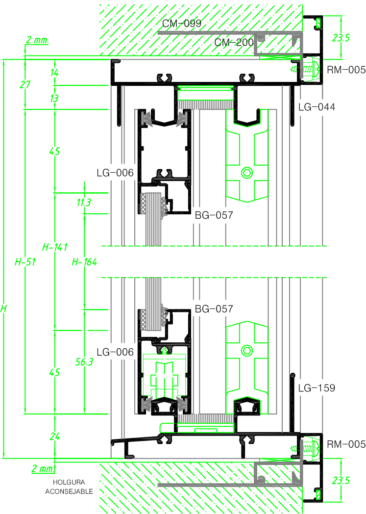
CORTE VERTICAL
