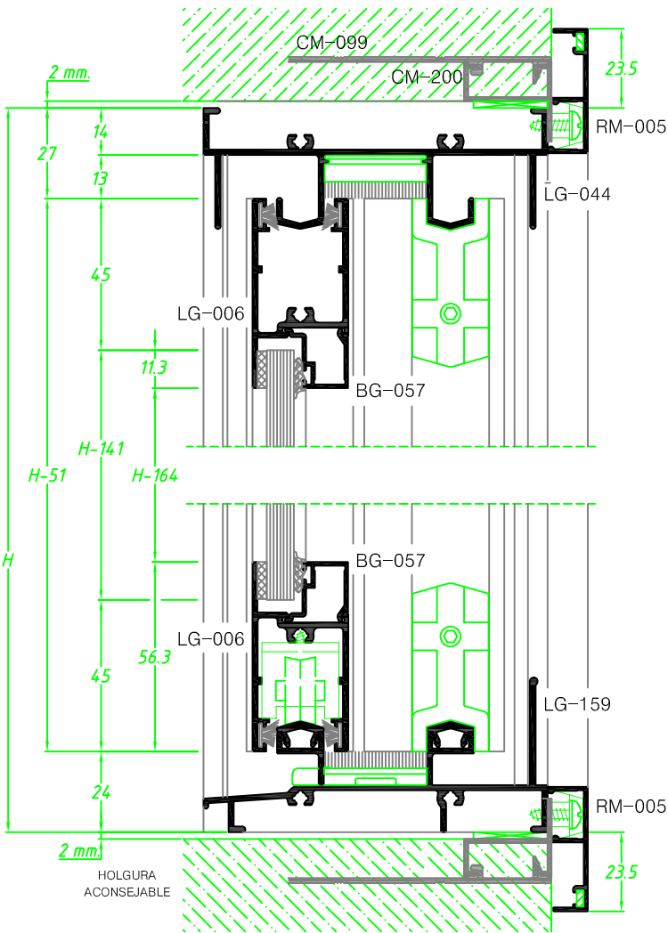
CORTE VERTICAL
