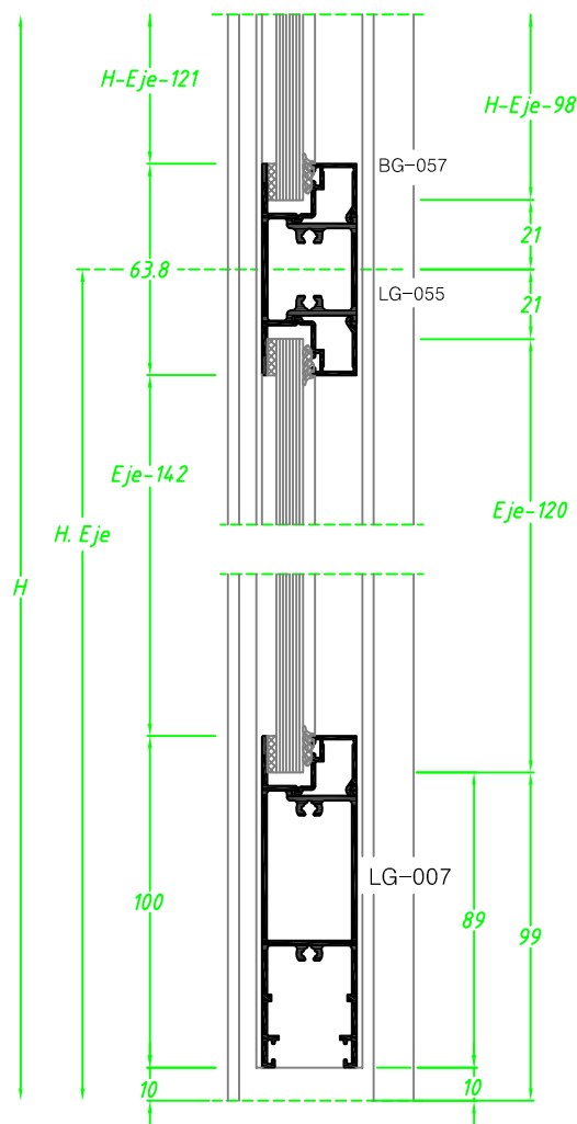
CORTE VERTICAL
