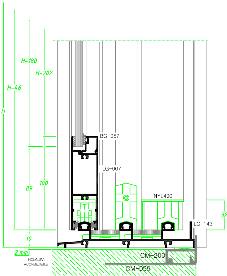
CORTE VERTICAL
