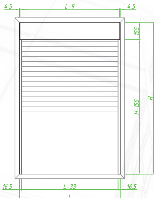
VISTA INTERIOR FRONTAL
