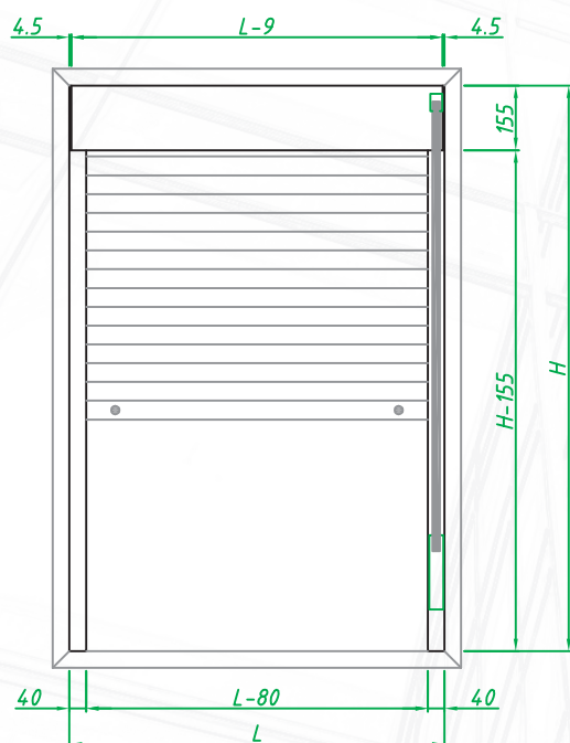
VISTA INTERIOR FRONTAL
