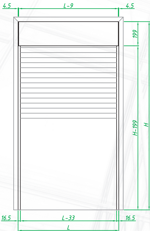
VISTA INTERIOR FRONTAL
