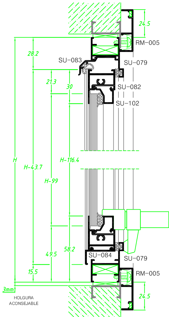
CORTE VERTICAL
