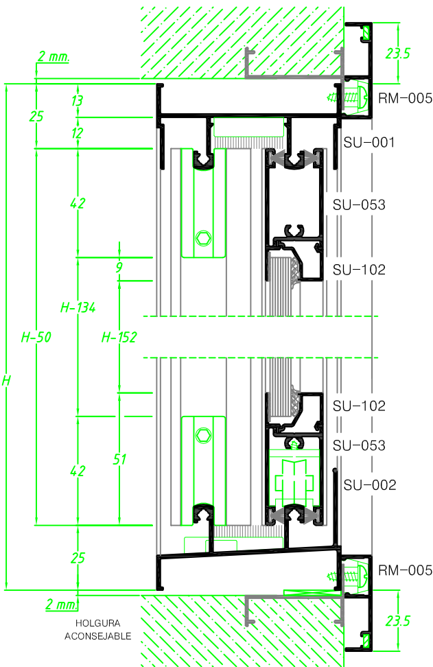
CORTE VERTICAL
