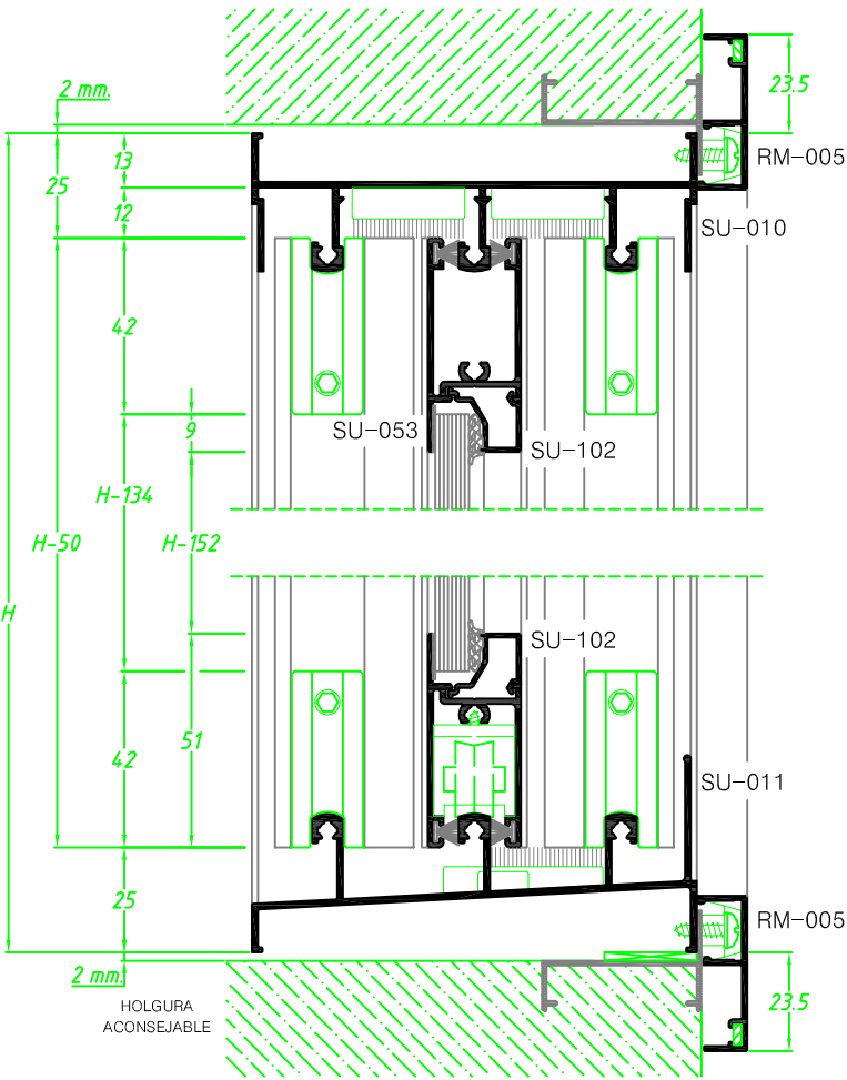
CORTE VERTICAL
