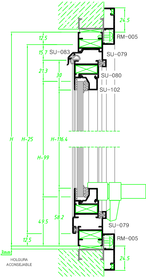
CORTE VERTICAL
